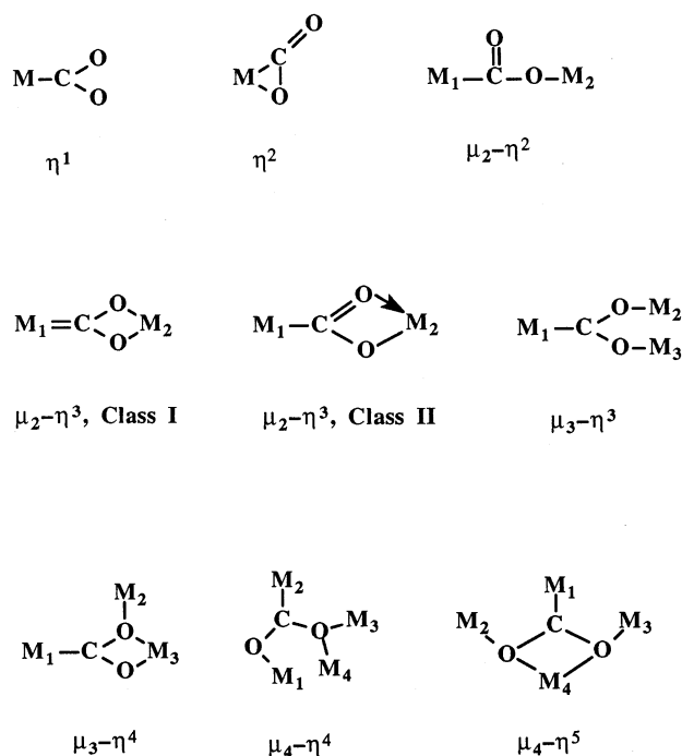
Fig. 1. Structural types of metal-CO 2 complexes.
